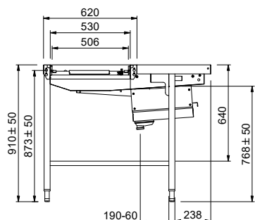
Factory mounted waste rack
